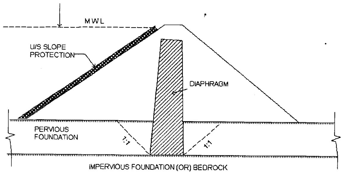
Type C- Diaphragm Type
