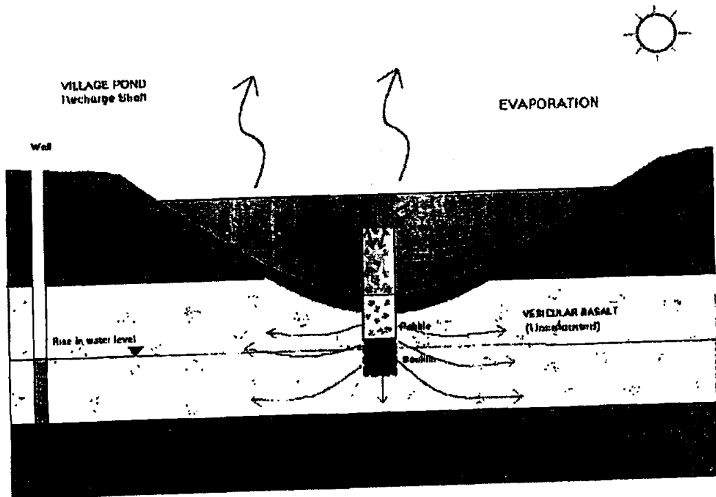
Recharge Shafts in a Village Pond
