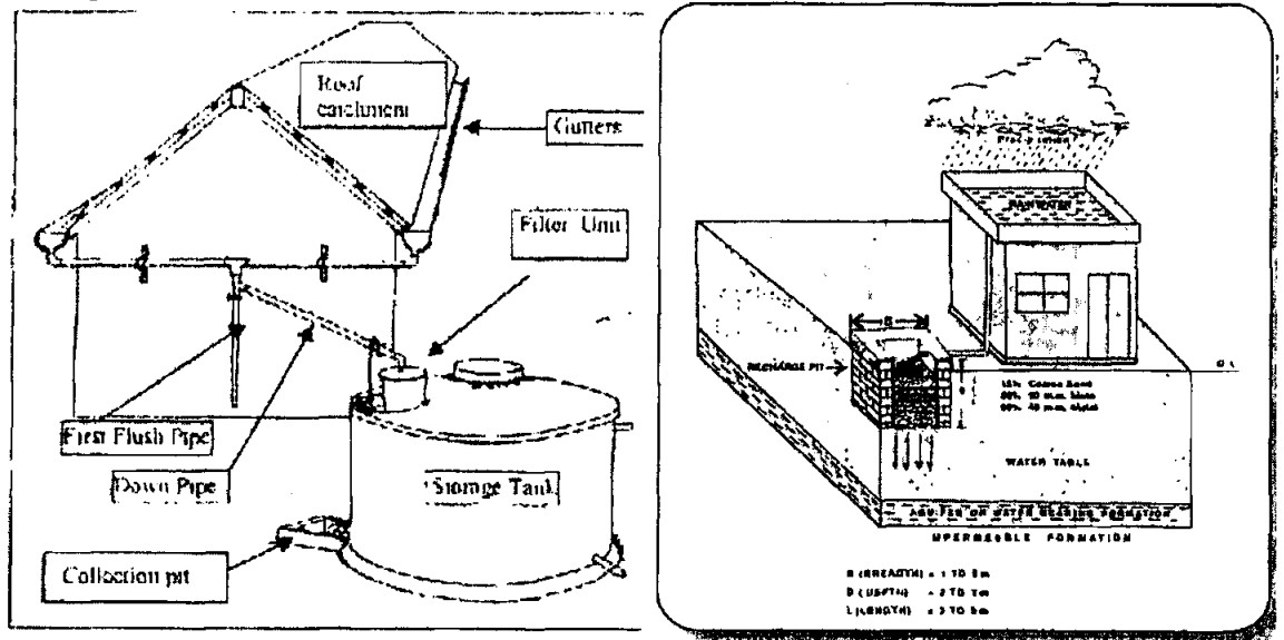
A Typical Rainwater Harvesting System
