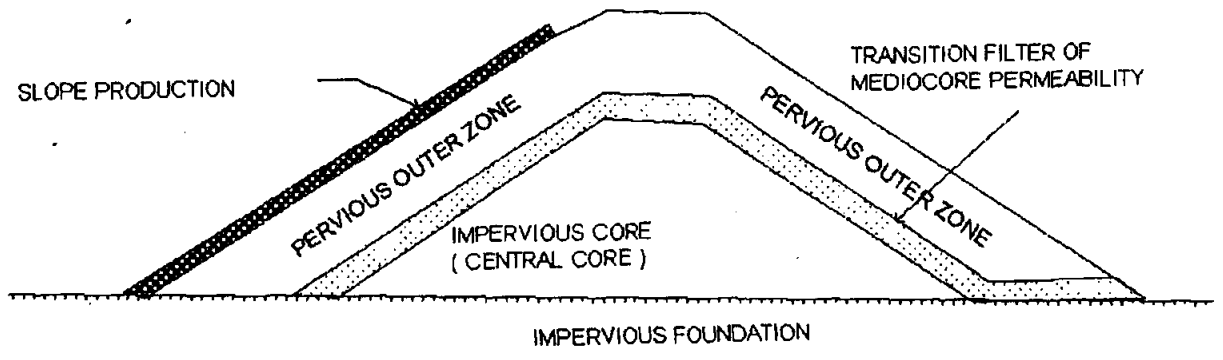
Type B -Zoned Type
